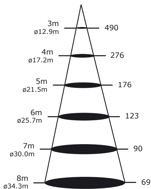
F04T200 - 130°
