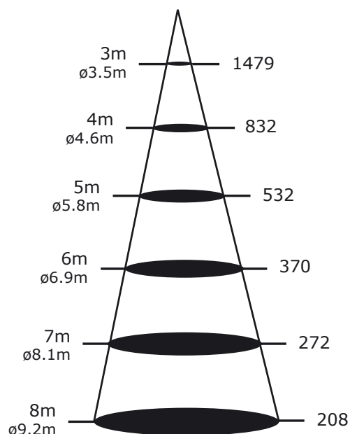
F04T200 - 60°
